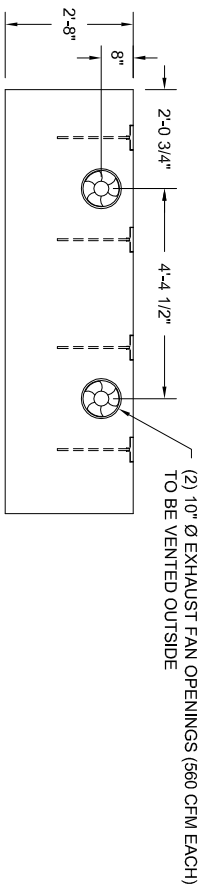
PLAN VIEW
